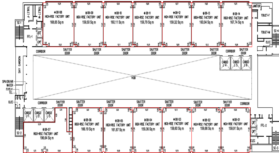
3.9 9 th storey plan indicating the location of Common Corridors
